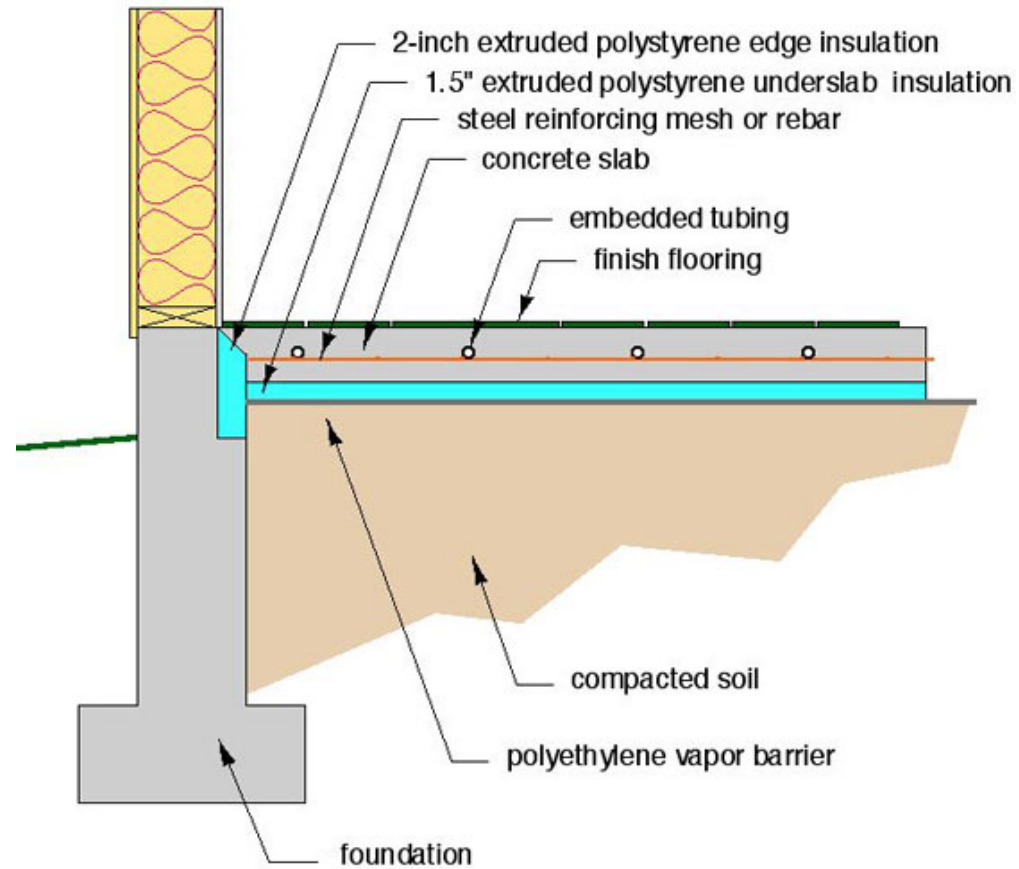
Slab Construction detail
